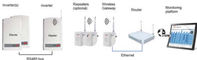
Figure 3: Multiple inverters, wired connection
